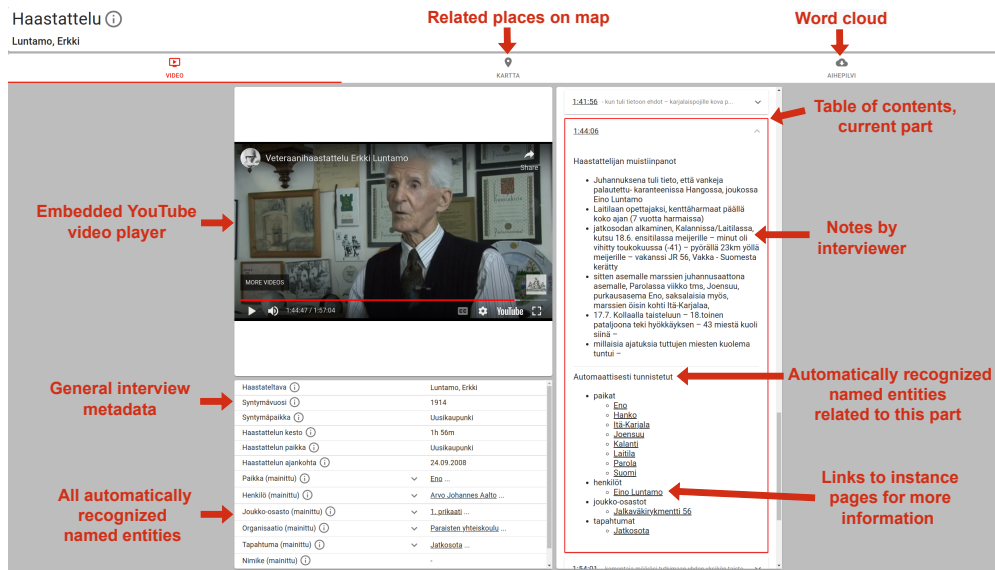
Figure 3: A video page with dynamic table of contents functionalities, provided by the portal.
