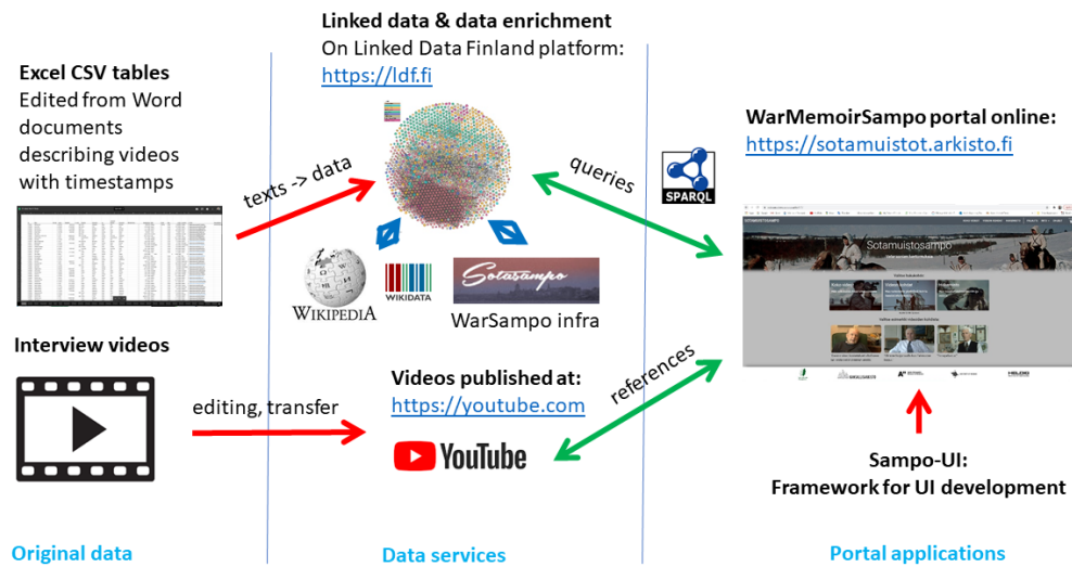
Figure 1: Publication pipeline from source data to the semantic video viewing portal online.
