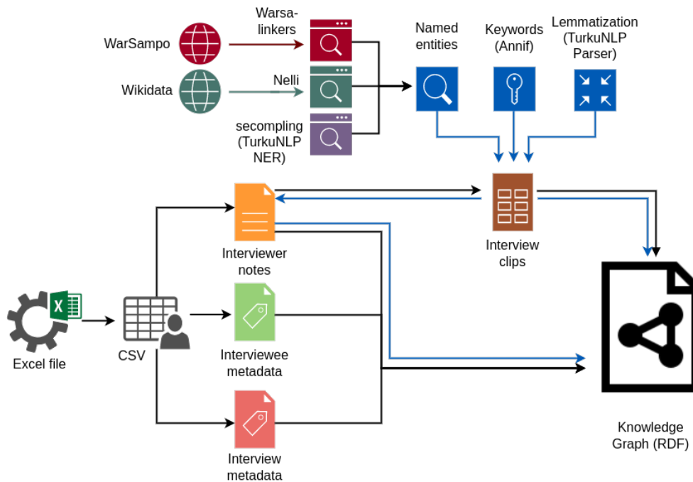
Figure 2: Overview of the data extraction and enrichment pipeline
